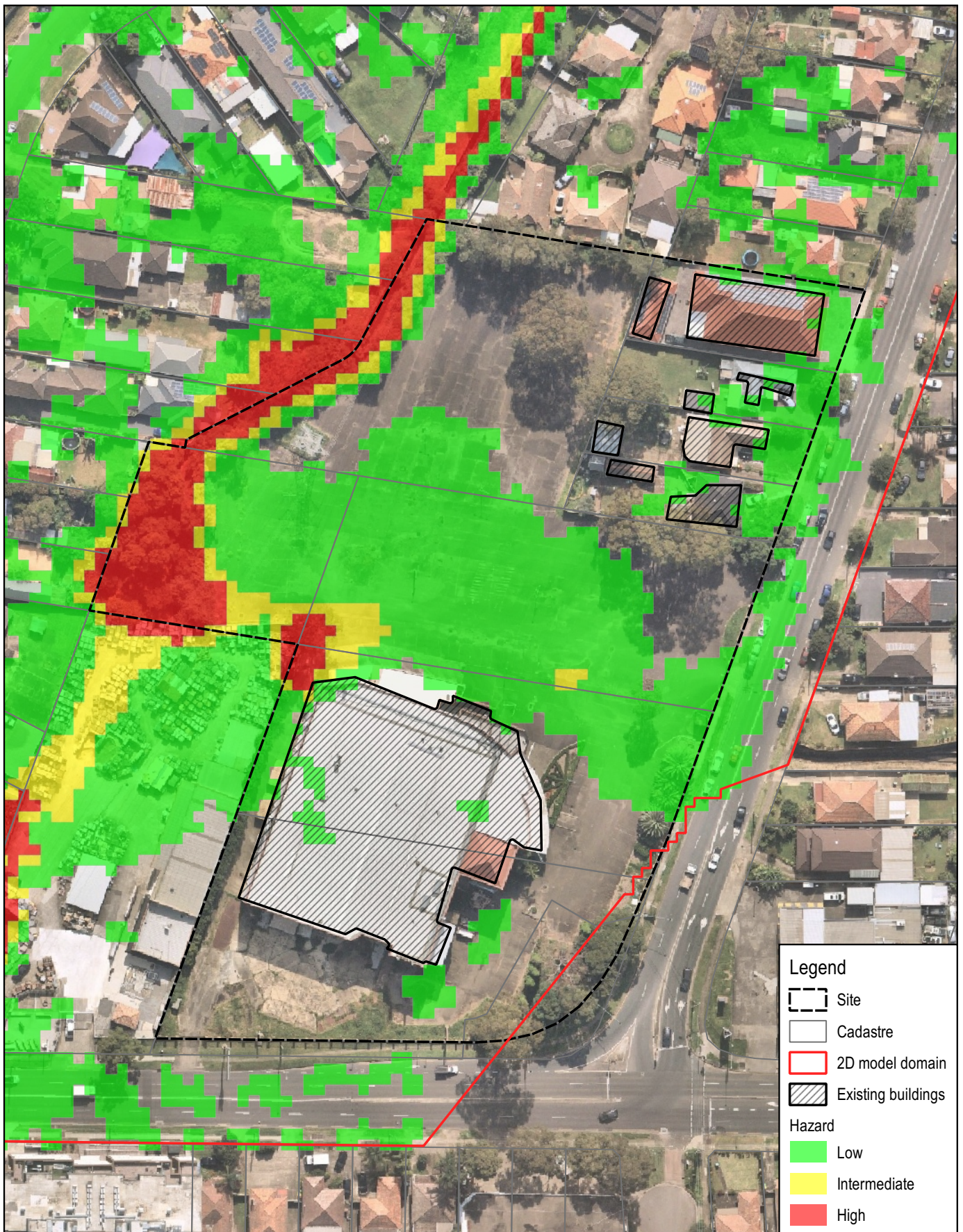
Title: PRE-DEVELOPMENT 1% AEP PROVISIONAL FLOOD HAZARD PLAN - 50% BLOCKAGE
