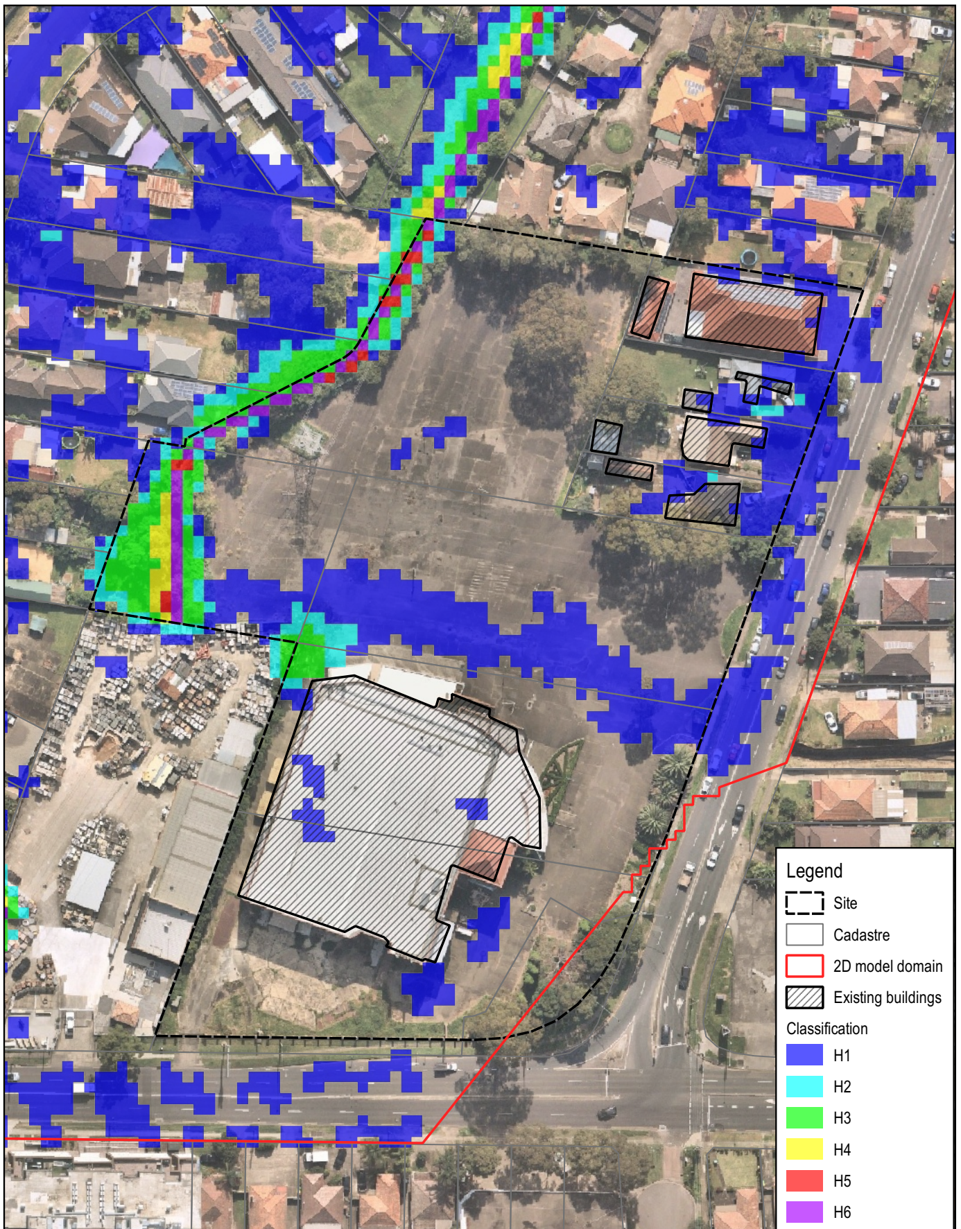
Title: PRE-DEVELOPMENT 1% AEP FLOOD HAZARD VULNERABILITY PLAN - 0% BLOCKAGE
