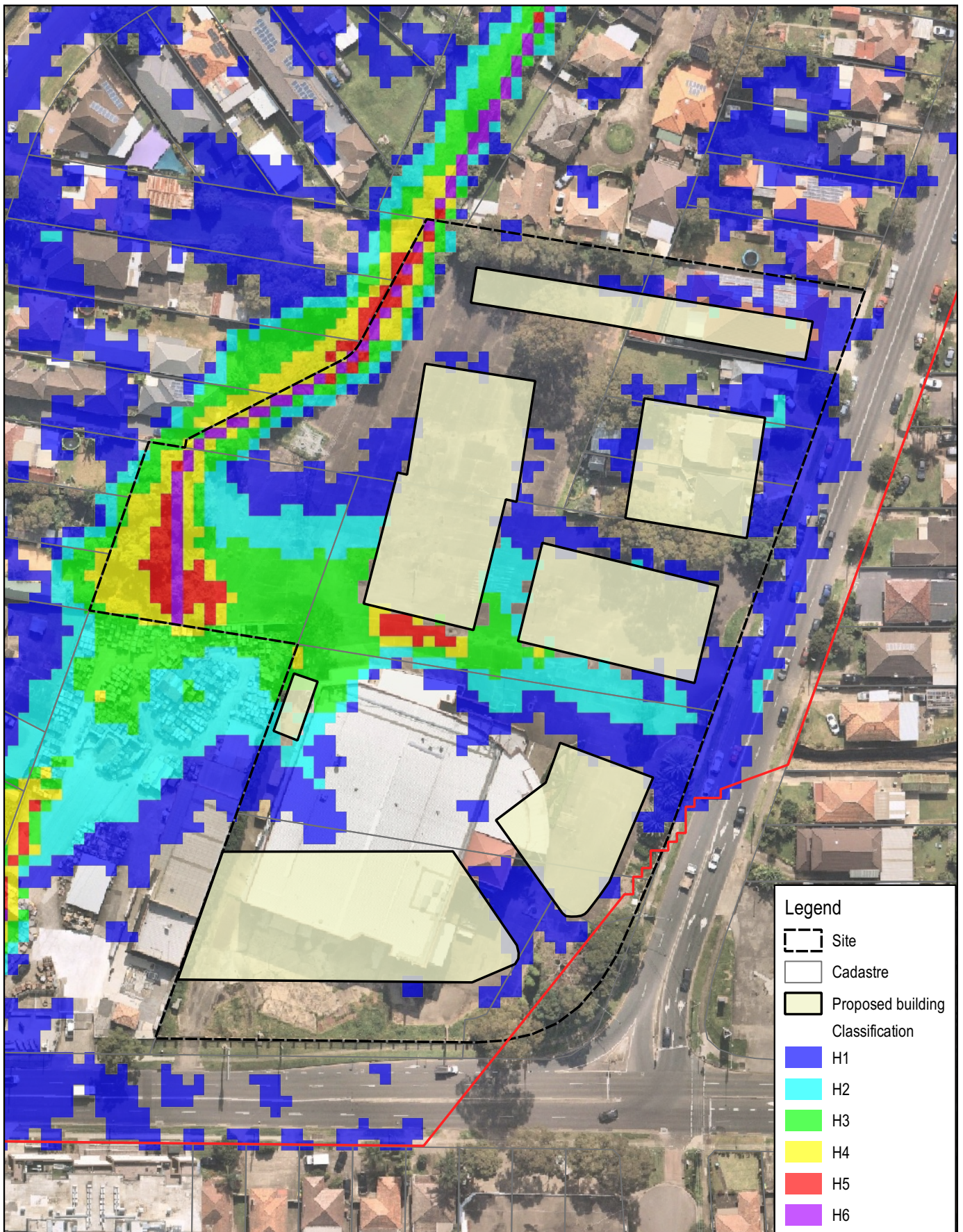
Title: POST-DEVELOPMENT 1% AEP FLOOD HAZARD VULNERABILITY PLAN - 50% BLOCKAGE
