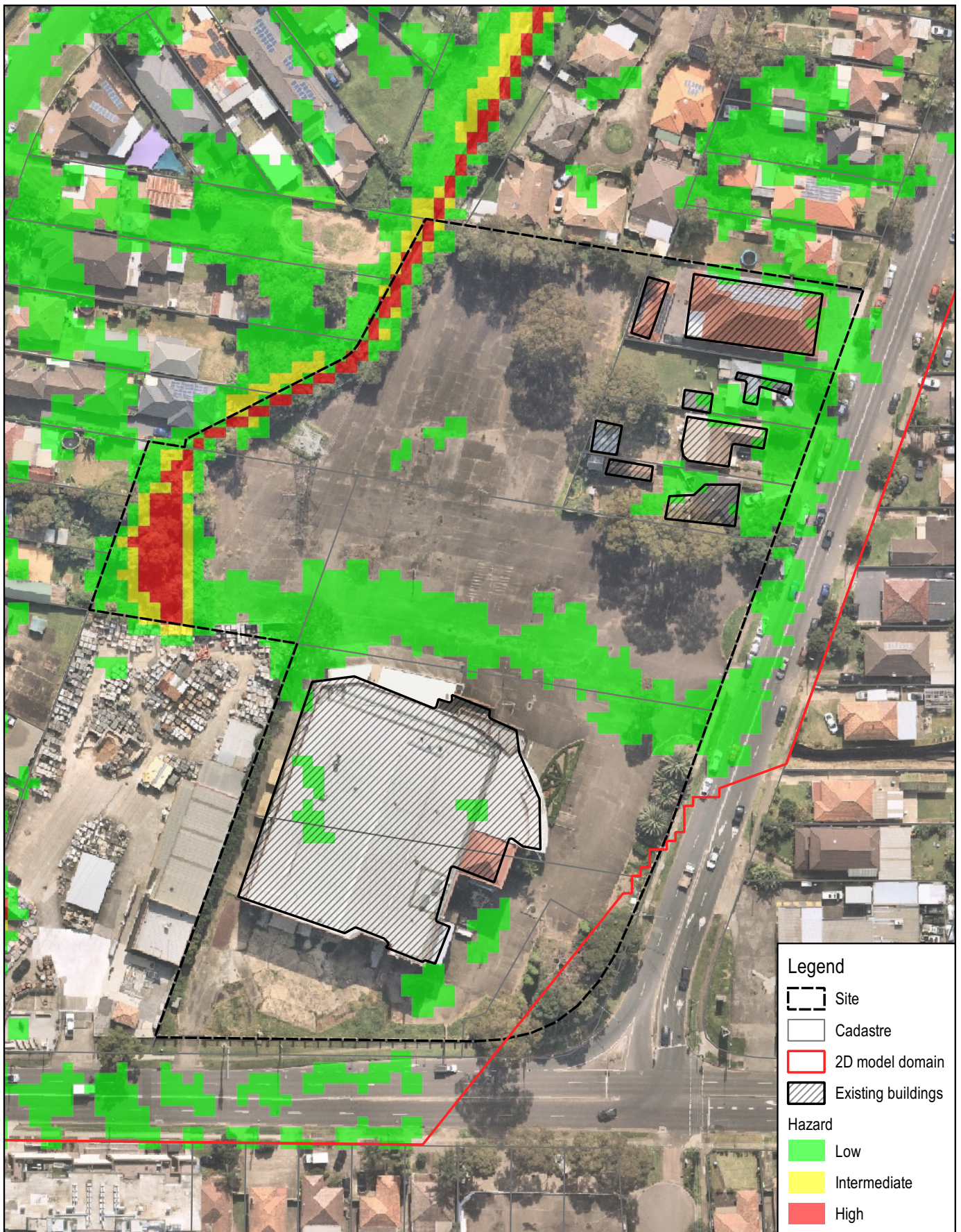
Title: PRE-DEVELOPMENT 1% AEP PROVISIONAL FLOOD HAZARD PLAN - 0% BLOCKAGE
