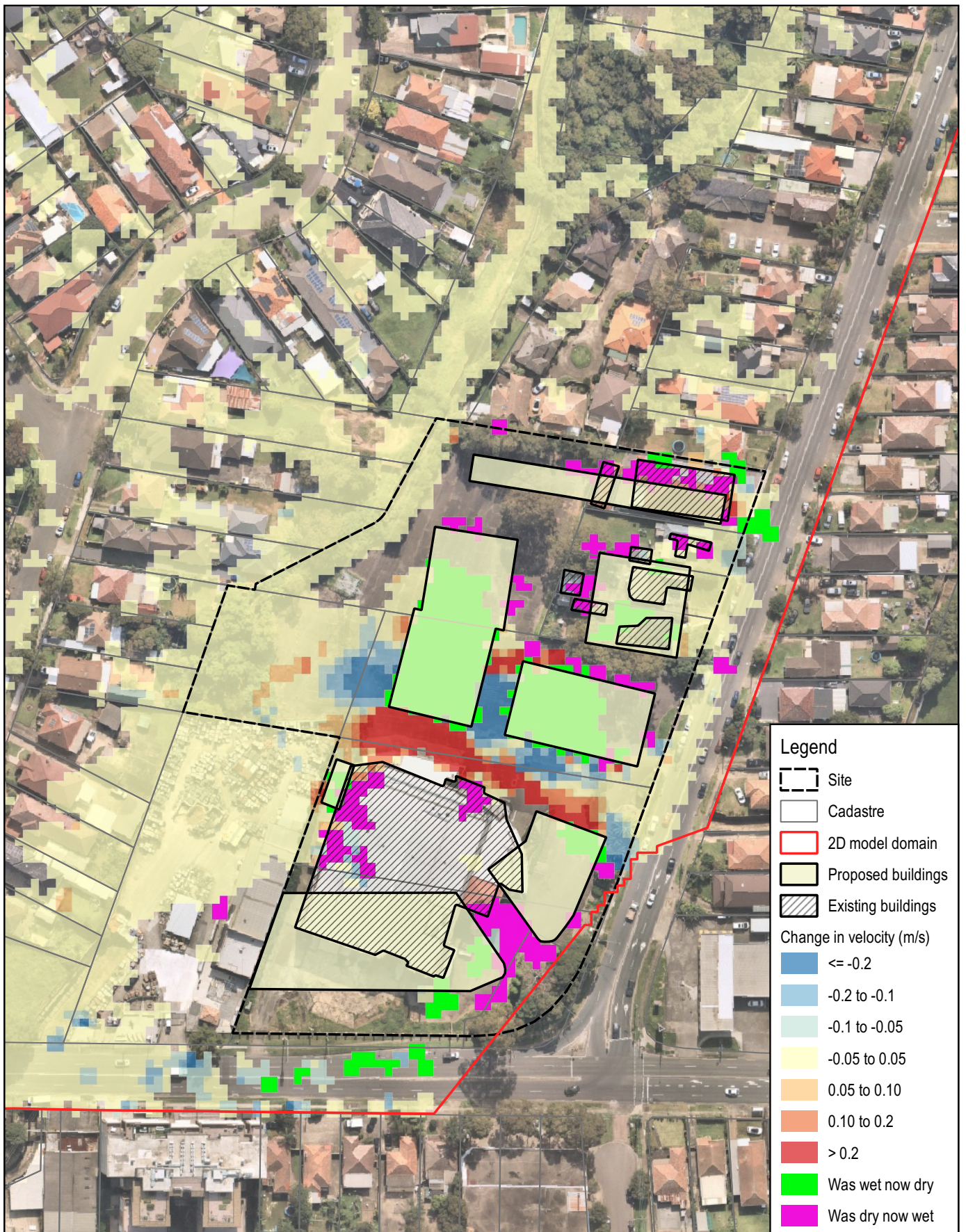
Title: POST-DEVELOPMENT 1% AEP FLOOD VELOCITY DIFFERENCE PLAN - 50% BLOCKAGE
