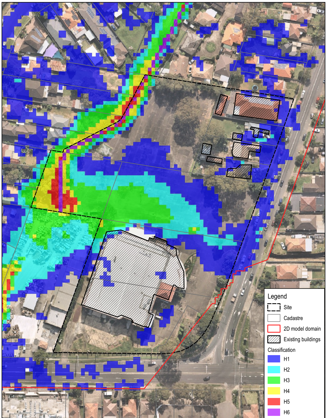
Title: PRE-DEVELOPMENT 1% AEP FLOOD HAZARD VULNERABILITY PLAN - 50% BLOCKAGE
