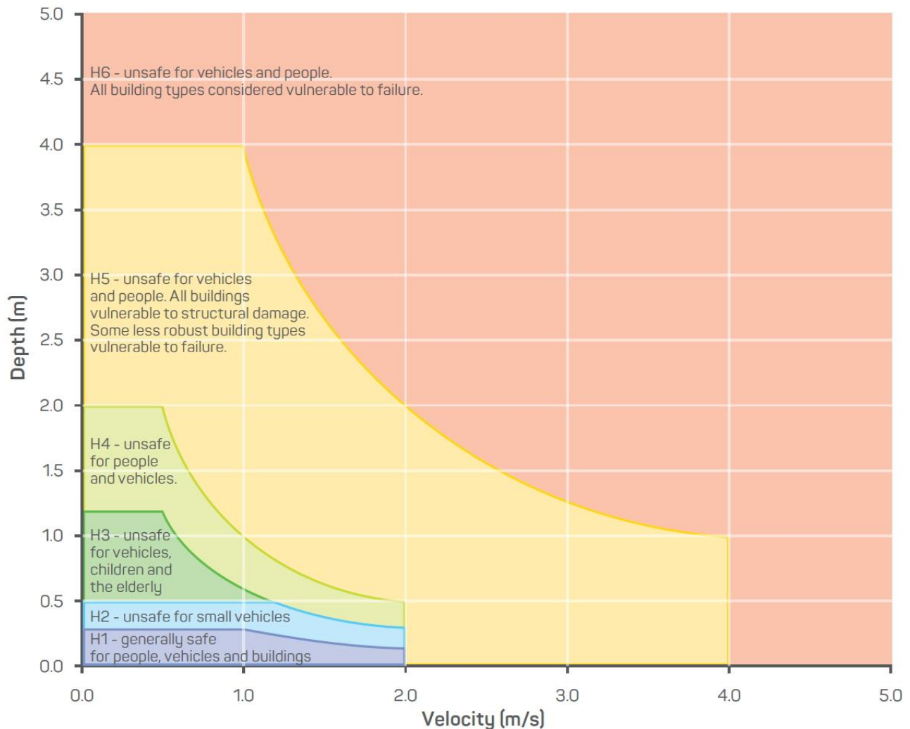
Figure 2: Hazard vulnerability classification (AIDR 2017).
